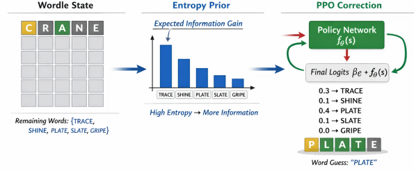
Figure 1. Overview of the entropy-guided PPO approach. Expected information gain from each guess is incorporated into the policy to guide action selection.
