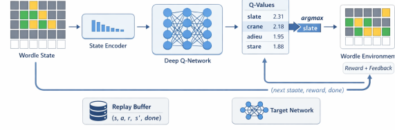
Figure 3. DQN-based Wordle approach
