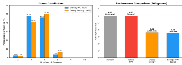
Figure 10. Left: distribution of guess counts for entropy-guided PPO and greedy entropy. Entropy-guided PPO shifts probability mass toward shorter solutions (3–4 guesses) and reduces longer games. Right: average number of guesses across agents, where entropy-guided PPO achieves the lowest average, outperforming both greedy entropy and vanilla PPO, indicating more efficient policies.
