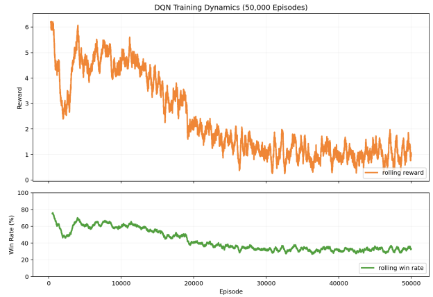
Figure 5. DQN training dynamics over 50,000 episodes. While early performance is relatively strong due to high exploration, both reward and win rate degrade as training progresses and \epsilon decays, ultimately converging to a suboptimal policy. This highlights the difficulty of learning effective strategies in Wordle using value-based methods with standard reward shaping.
