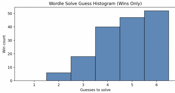
Figure 14. Distribution of guesses required by the DQN agent (wins only). The distribution is skewed toward higher guess counts, indicating inefficient policies and poor convergence compared to PPO-based methods.
