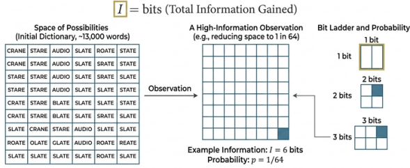
Figure 4. Explanation of precomputed entropy matrix. Across the entire Wordle vocabulary, we compute the entropy \sum p(x) \log(\frac{1}{p(x)}) to find total bits of information gained from each guess. This value measures how effectively a guess partitions the remaining solution space.
