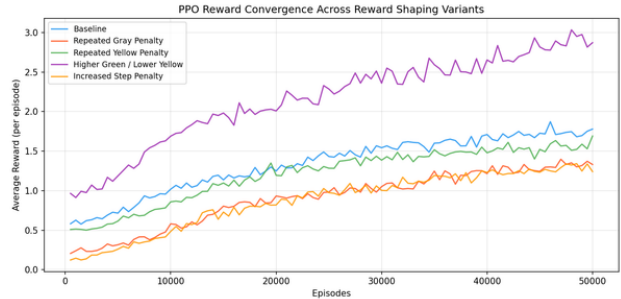
Figure 6. PPO reward convergence across different reward shaping variants. Increasing the reward for correctly placed letters (green) leads to faster and higher convergence, while penalizing repeated gray letters and increasing step penalties result in slower learning and lower asymptotic performance.
